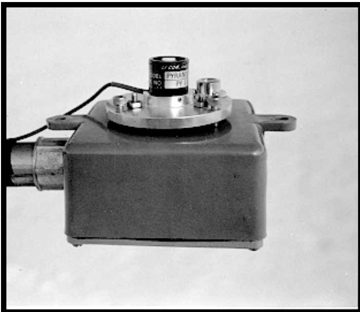
A76-I Mount with Pyranometer
